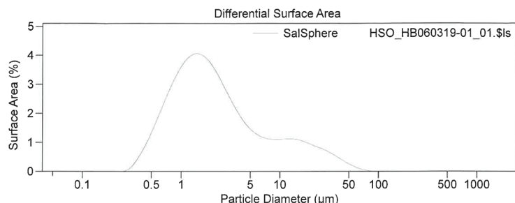
Figure 6: Particle size analysis of SS HSO showing an average diameter of over 1 micron using the Beckman Coulter LS Particle Size Analyzer.
